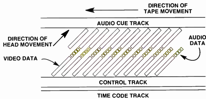
Figure 1. The D-1 magnetic footprint. Notice guardbands between the tracks and a constant azimuth angle on all tracks. (The azimuth is parallel to the end of the recorded tracks.)
