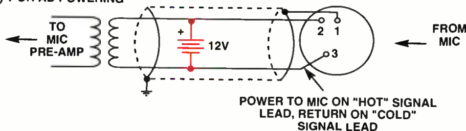
Figure 2. In (A), phantom power sends the same DC voltage up both wires of a balanced audio circuit. In (B), T-power sends power up just one wire. In both cases, the same wires that carry AC audio signals away from the mic carry DC power to it.
